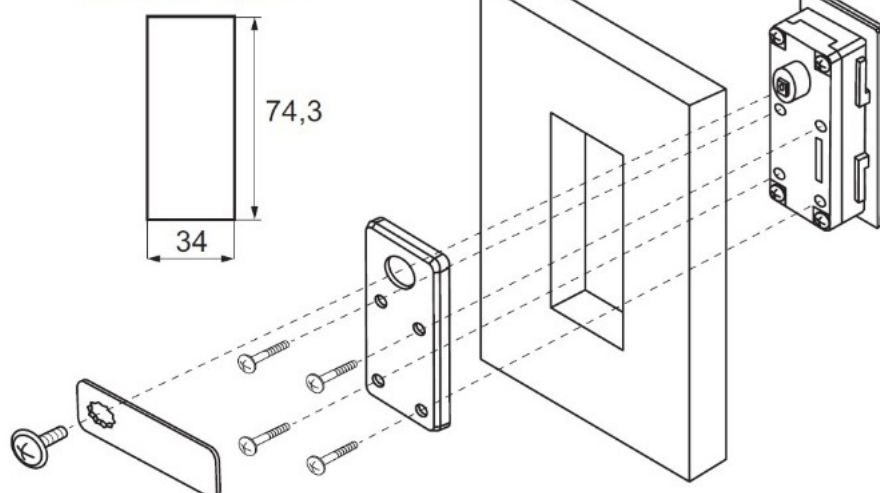
Drilling template for wooden panel
